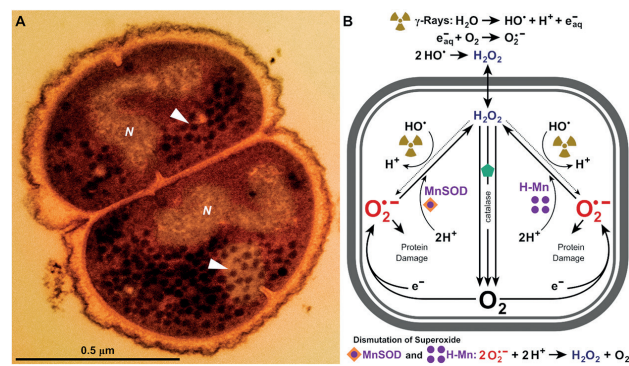
Figure 1: Deinococcus radiodurans antioxidant defenses. (A) Electron-dense granules are highly enriched in Mn 2+ and phosphate precursors of Mn antioxidants, visualized by transmission electron microscopy (TEM), identified by arrows inside a dividing. The 4–8 identical genomes per cell in D. radiodurans are condensed into nucleoids (N) wherein the chromosomes and plasmids are highly recombinogenic. Scale bar 0.5 μm. (B) Ionizing radiation-driven reactions that generate reactive oxygen species (ROS) and cellular mechanisms related to dismutation of superoxide (O 2 •- ) by Mn-dependent superoxide dismutase (MnSOD) and Mn antioxidants, illustrating the two complementary catalysts of superoxide defense, MnSOD and Mn antioxidants (H-Mn). Importantly, O 2 •- damages proteins, but not DNA. (the figure is adapted from [10])
